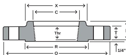
THREADED
