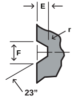
GROOVE DETAIL
