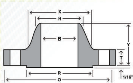
WELD NECK
